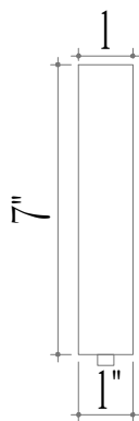
LEG DETAIL
