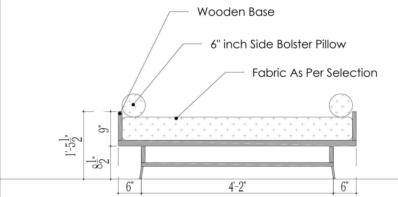
LEG DETAIL
