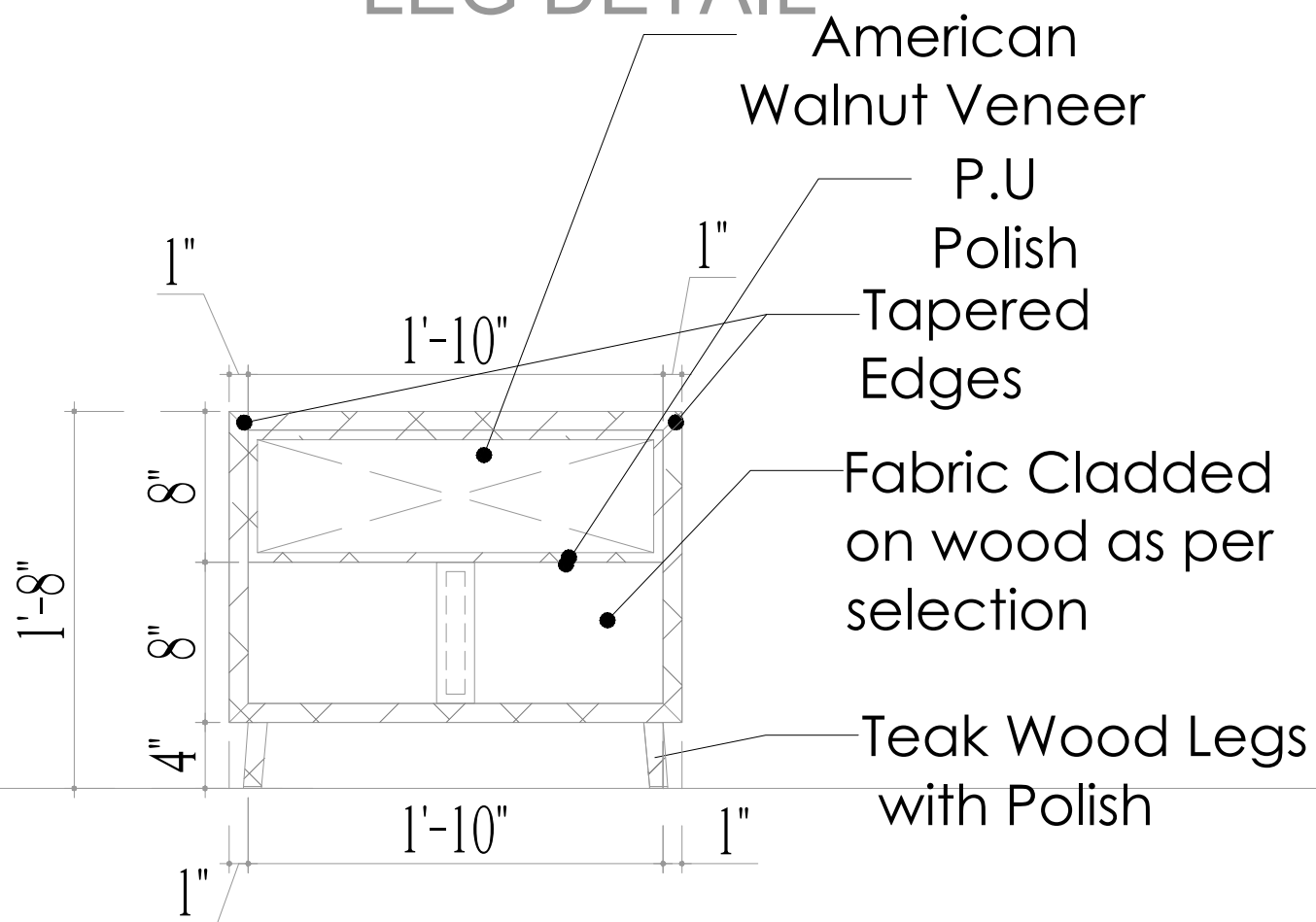
FRONT & SIDE ELEVATION
