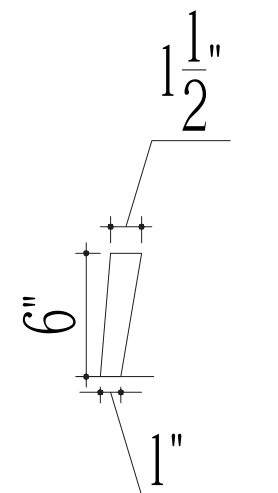
LEG DETAIL
