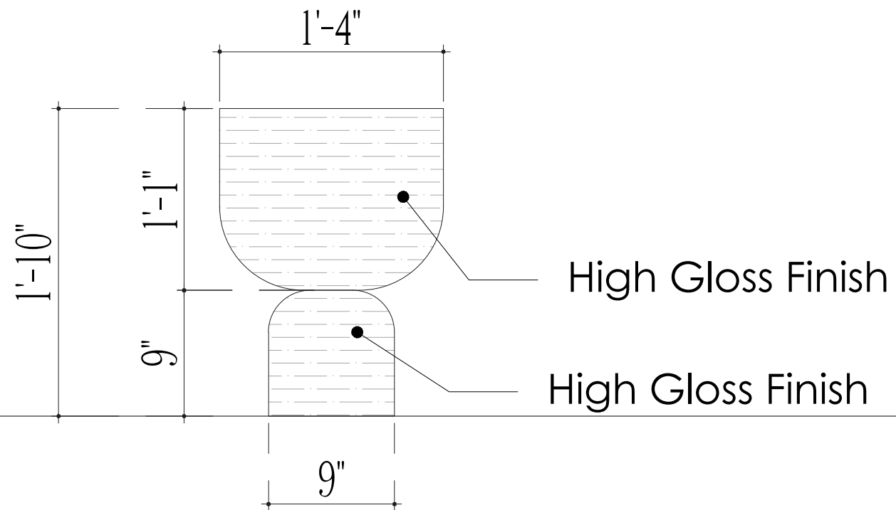
SIDE ELEVATION
