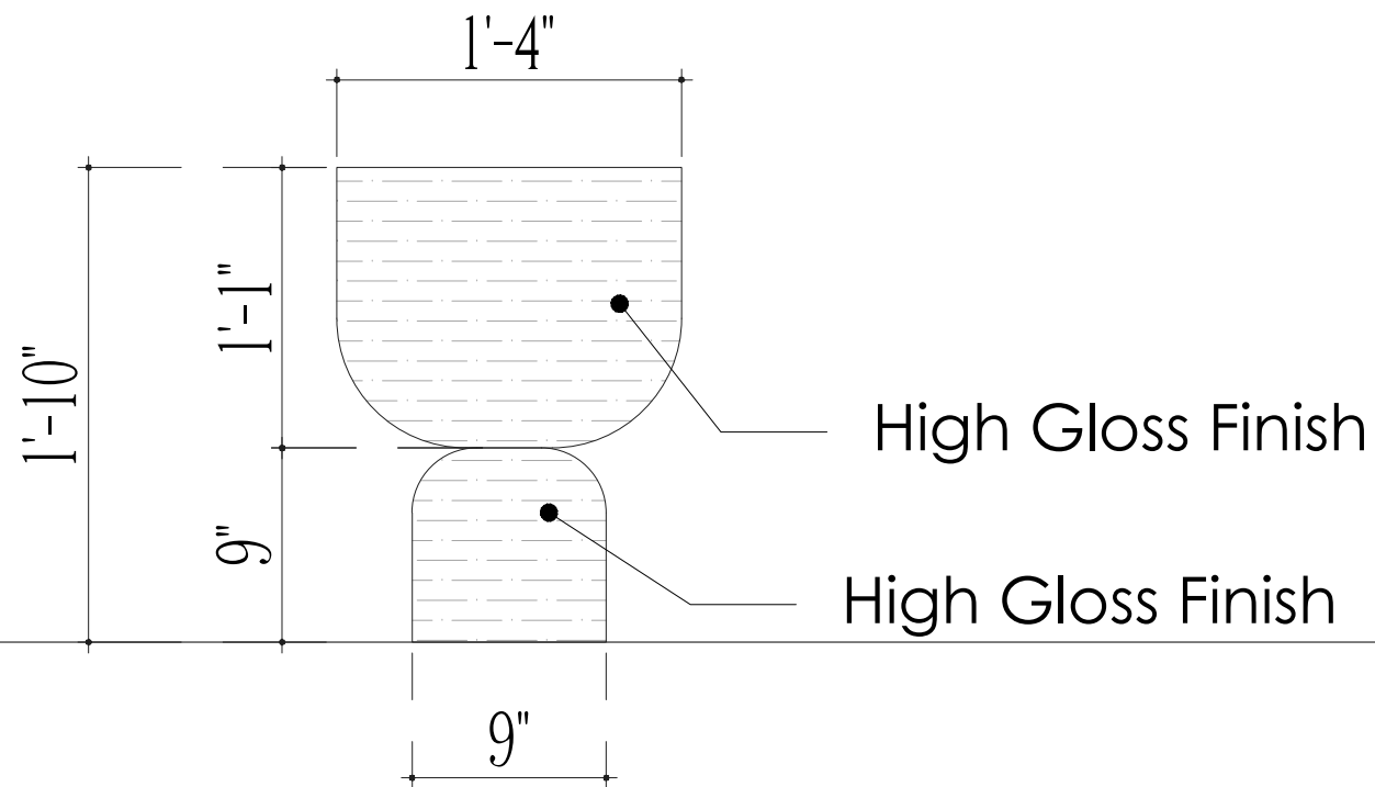
FRONT ELEVATION
